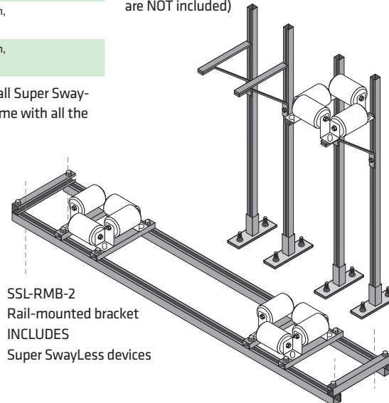
SSL-FMB-48 Floor-mounted bracket (Super SwayLess devices are NOT included)
