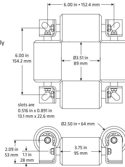
SSL-FMB-48 Floor-mounted bracket (Super SwayLess devices are NOT included)
