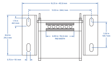
Installation footprint RB625
