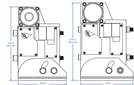
H/W Dimensions for RB500 and RB625
