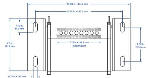
Installation footprint RB625
